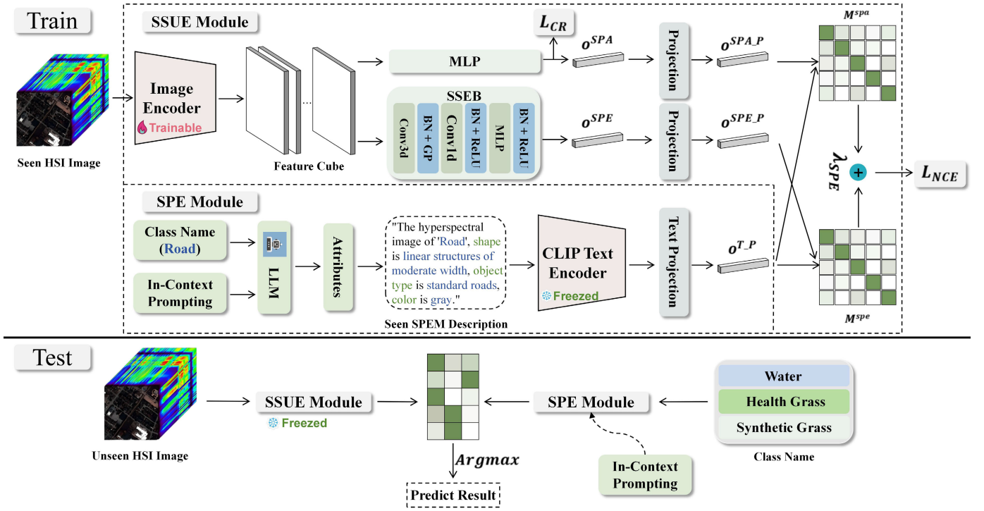
Fig. 2. Framework of the proposed SpectralZero. The SPE module encodes rich natural language descriptions into semantic features and projects them into both spatial and spectral embedding spaces. The SSUE module decouples image features into spatial and spectral components, which are then aligned with the corresponding semantic features. The similarity matrices from the two aligned spaces are fused and used to compute the loss during training. During testing, classification is performed by selecting the class index corresponding to the maximum value in the fused similarity matrix.
