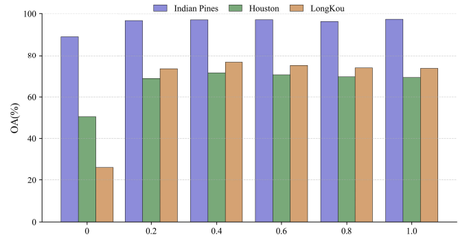
Fig. 12. Experimental results on the three datasets under different loss fusion weights.
