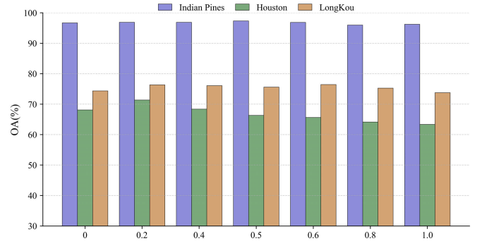
Fig. 11. Experimental results on the three datasets under different spectral similarity fusion coefficients.
