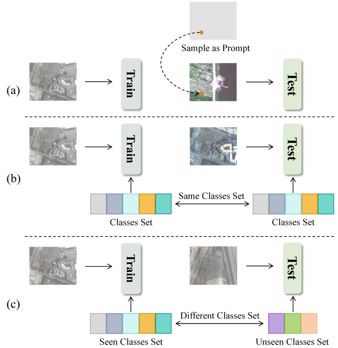
Fig. 1. Difference among three models. (a) Prompt learning-based zero-shot classification (such as HyperFree [29]), which still requires class-related samples as prompts for testing; (b) domain generalization (see [30]), which is conducted within the same dataset and category settings; and (c) text-guidance zero-shot classification (ours), where the train and test classes are disjoint, and the model identifies different land-cover categories through cross-class knowledge transfer.
